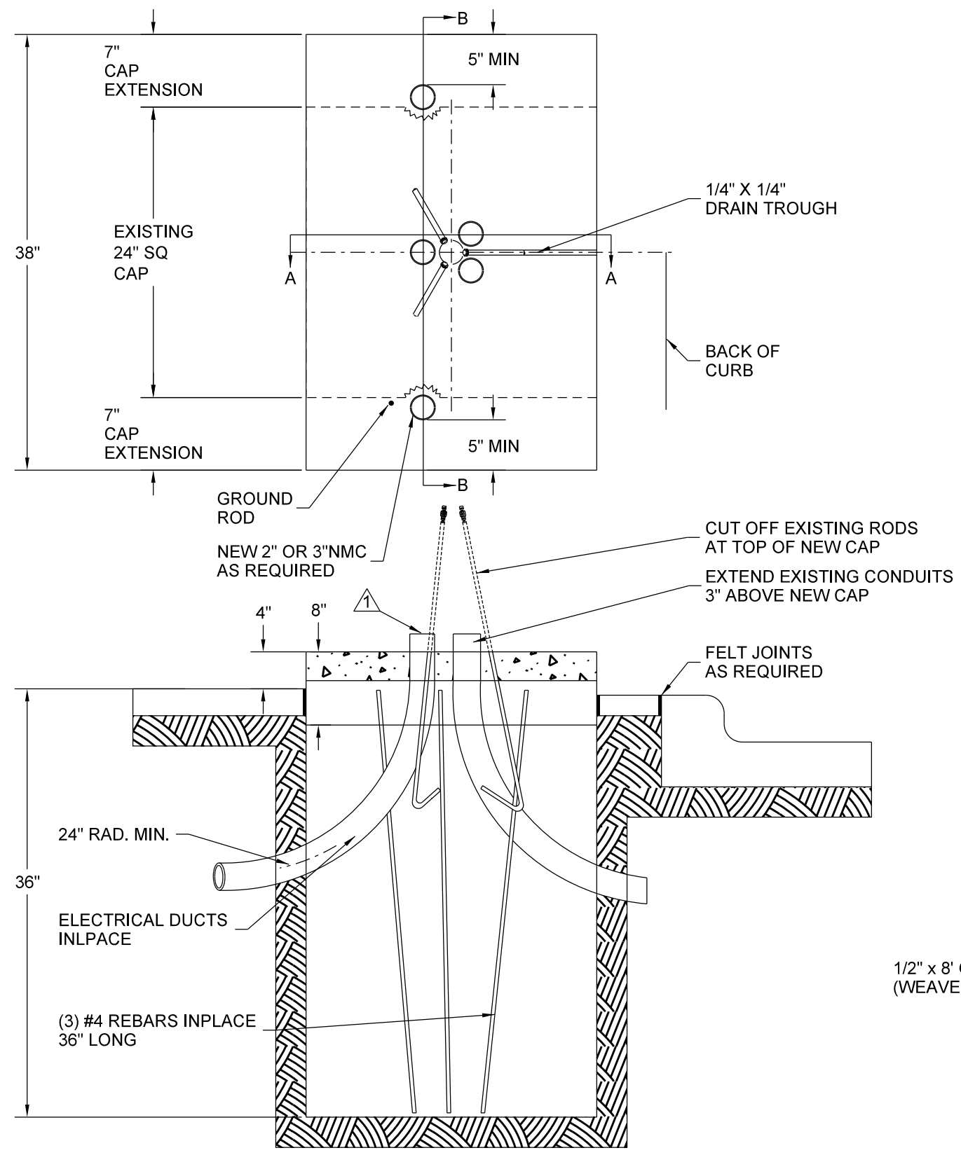
SECTION "A"
