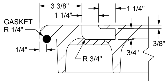
GASKET & PICK HOLE DETAIL
