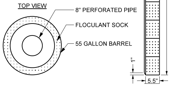
TYPICAL FLOCULANT SOCK
