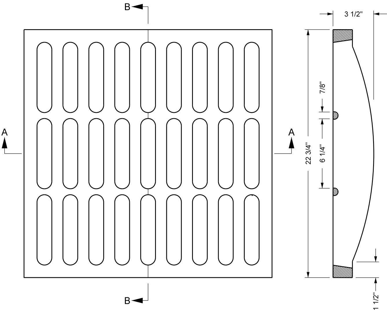
SECTION B-B
