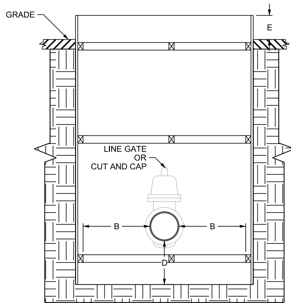
PROFILE VIEW
