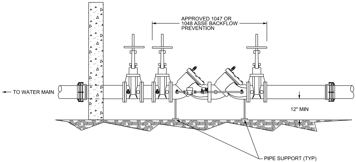
PROFILE VIEW
