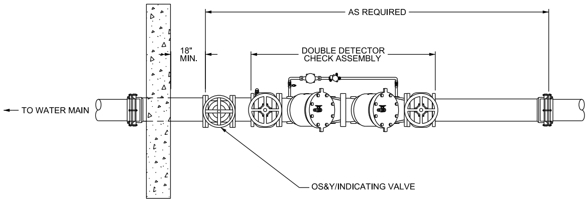
PLAN VIEW
