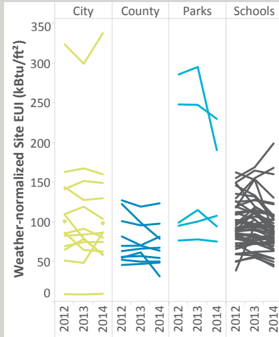
Figure 15. Weather-normalized site energy use intensity (kBtu/ft 2 ) by public entity from 2012 to 2014
