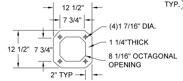
VIEW B-B (MAST ARM & SIGN ARM)
