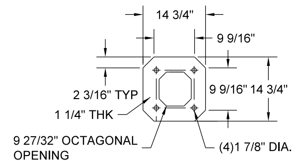
VIEW G-G
