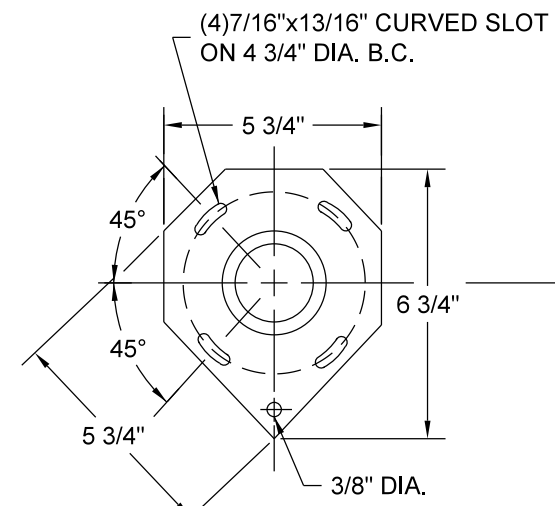
DETAIL D
