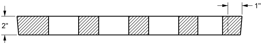
SECTION B-B
