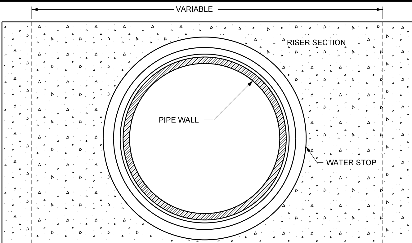
CORE DRILLED HOLE OR DOGHOUSE IN PRECAST RISER
