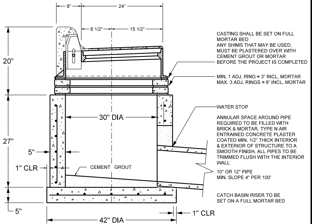
TYPICAL CATCH BASIN CONSTRUCTION, MINNEAPOLIS STANDARD
