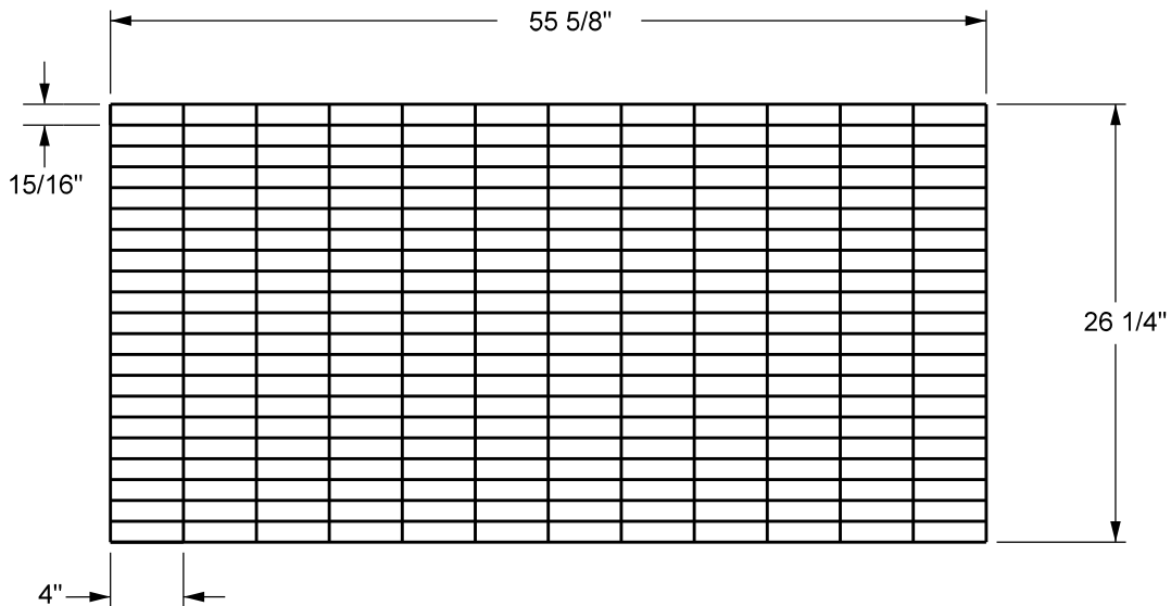
PANEL SECTION (3 PANELS = 1 SET) TOP VIEW
