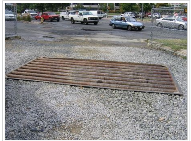
Example shaker rack installation. Source: Tetra Tech.
